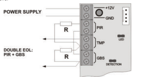
Example of wiring the JS-25 into the double EOL zone.
