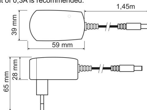
Fig.1. Dimension of power supply.
